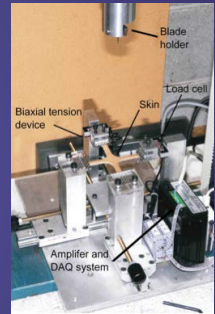
Biaxial tension device
